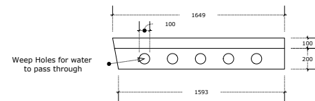
RCC Platform - Elevation
