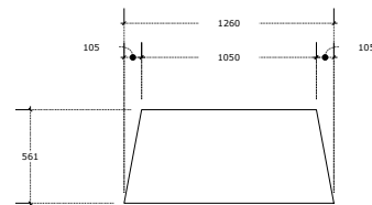
RCC Footing - Elevation
