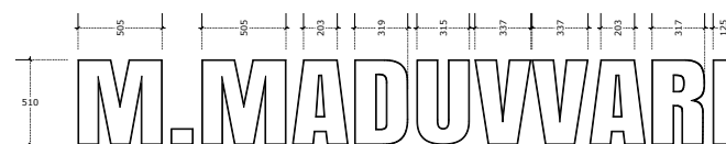
RCC LETTER - Elevation
