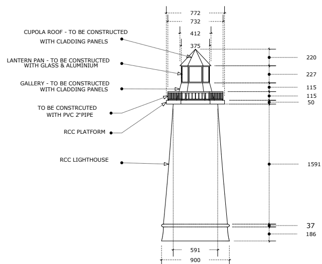
Lighthouse - Elevation
