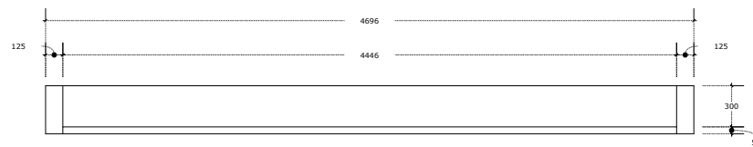
RCC Wall - Elevation
